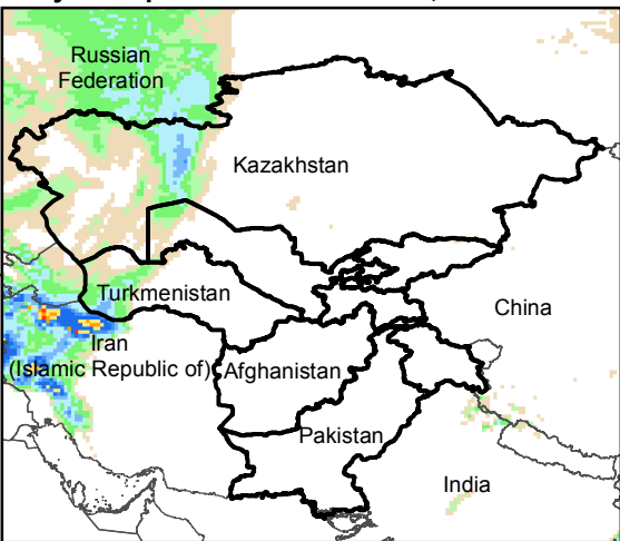
Daily Precip. Forecast for 10 Dec., 2017
