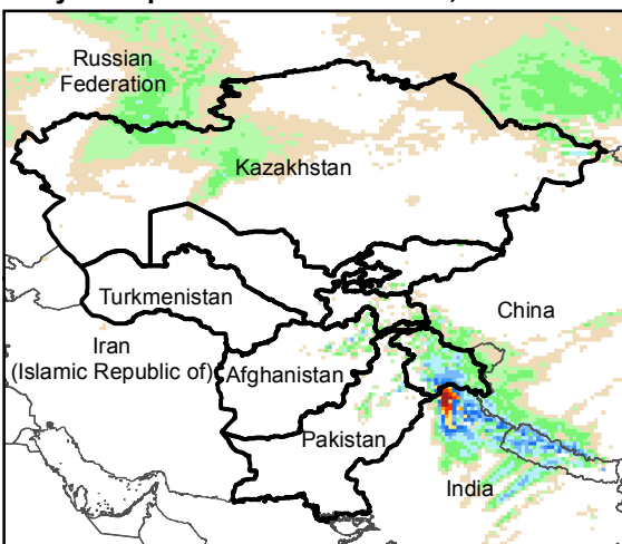
Daily Precip. Forecast for 12 Dec., 2017
