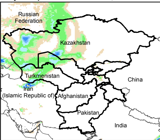
Daily Precip. Forecast for 11 Dec., 2017
