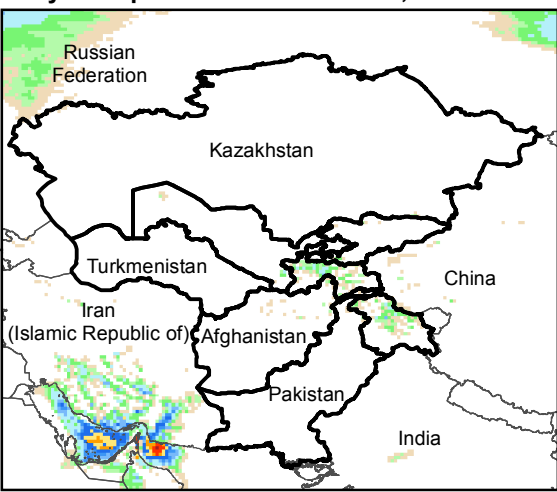
Daily Precip. Forecast for 16 Dec., 2017
