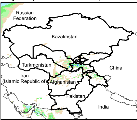
Daily Precip. Forecast for 18 Dec., 2017
