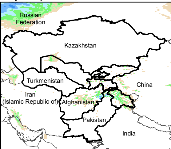
Daily Precip. Forecast for 17 Dec., 2017
