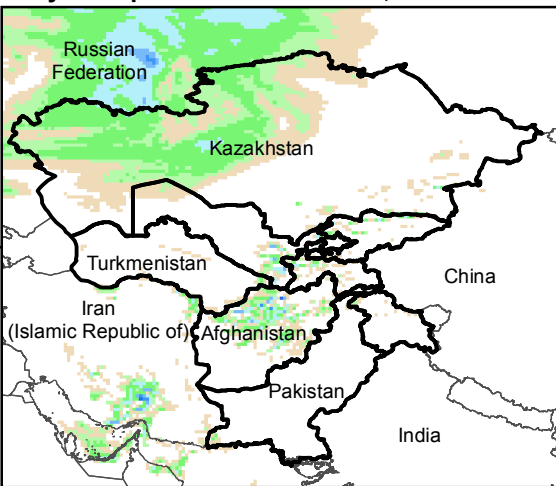
Daily Precip. Forecast for 11 Jan., 2018
