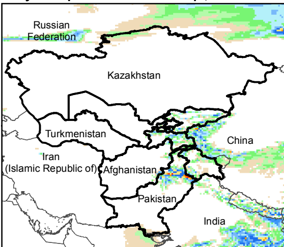
Daily Precip. Forecast for 17 Sep., 2018
