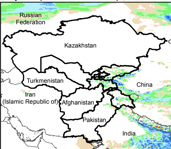
Daily Precip. Forecast for 16 Sep., 2018
