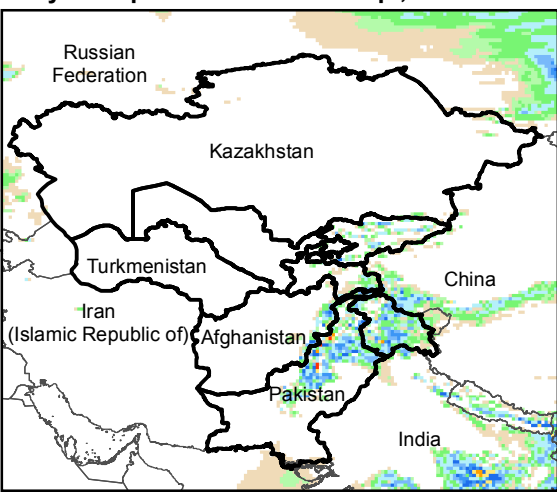
Daily Precip. Forecast for 15 Sep., 2018
