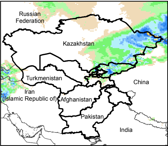
Daily Precip. Forecast for 3 Dec., 2018
