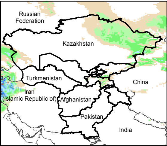
Daily Precip. Forecast for 4 Dec., 2018
