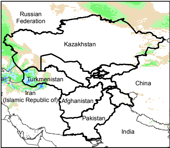
Daily Precip. Forecast for 5 Dec., 2018
