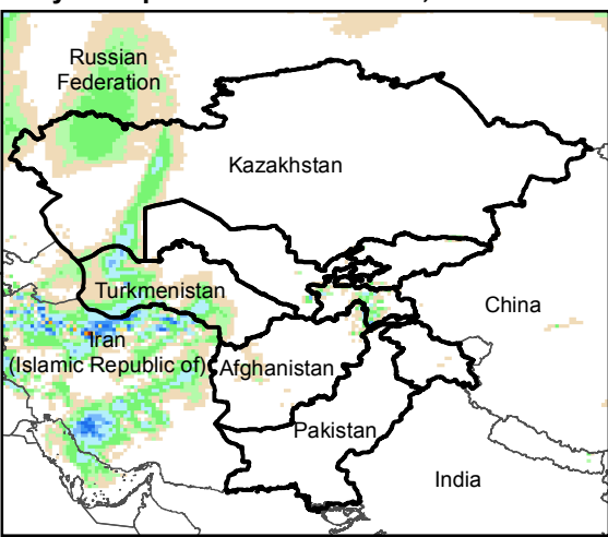
Daily Precip. Forecast for 7 Dec., 2018
