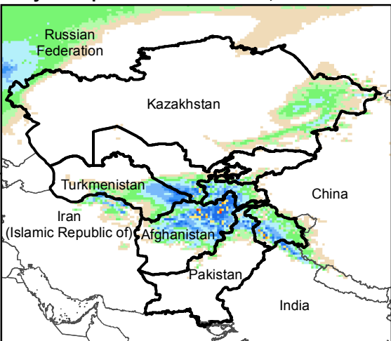
Daily Precip. Forecast for 7 Jan., 2019
