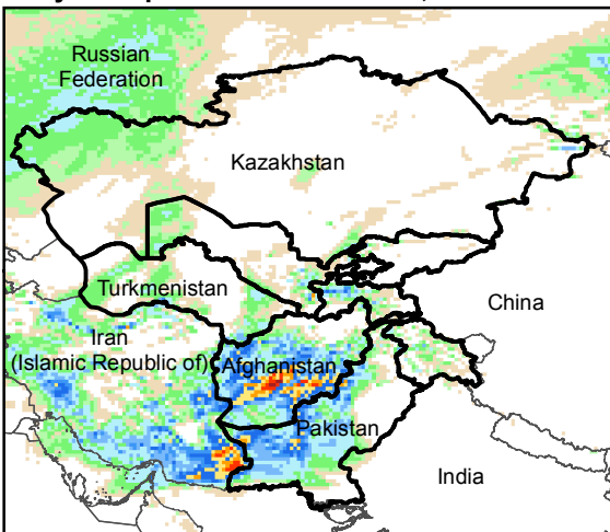
Daily Precip. Forecast for 4 Mar., 2019
