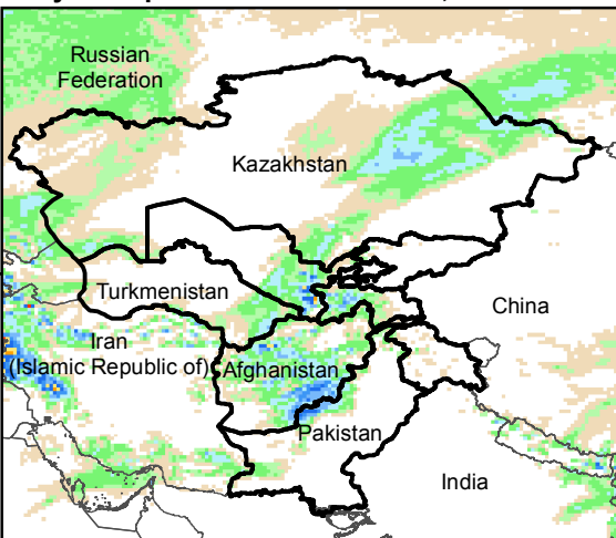
Daily Precip. Forecast for 3 Mar., 2019
