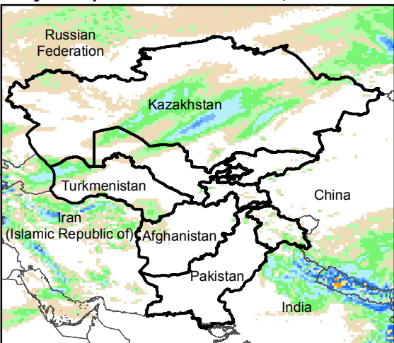
Daily Precip. Forecast for 2 Mar., 2019
