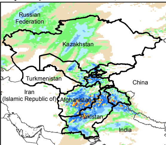
Daily Precip. Forecast for 5 Mar., 2019
