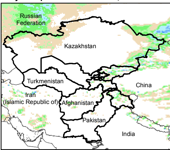
Daily Precip. Forecast for 6 Mar., 2019
