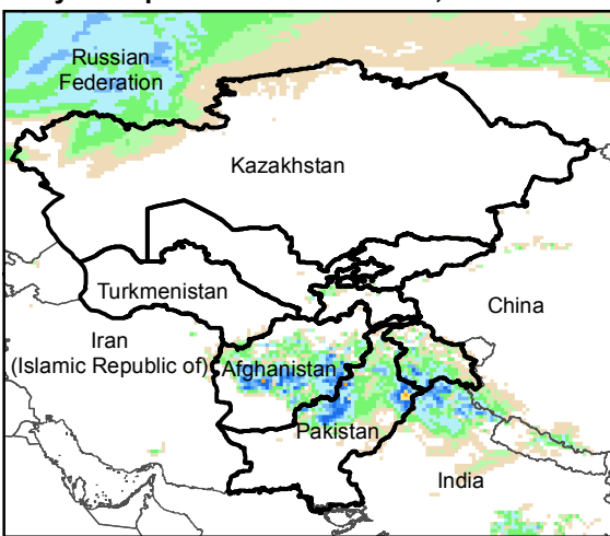
Daily Precip. Forecast for 11 Mar., 2019
