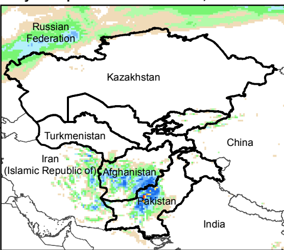
Daily Precip. Forecast for 10 Mar., 2019
