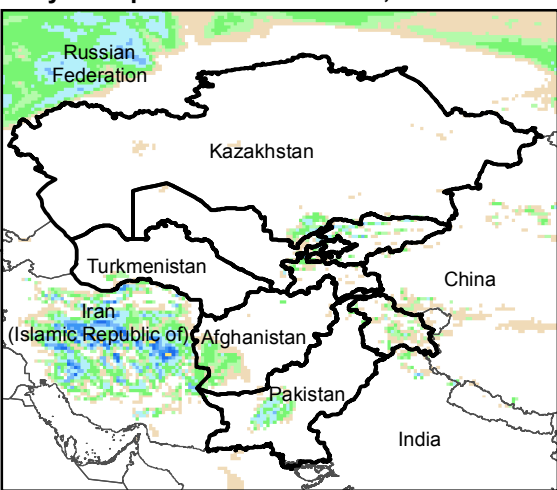
Daily Precip. Forecast for 9 Mar., 2019
