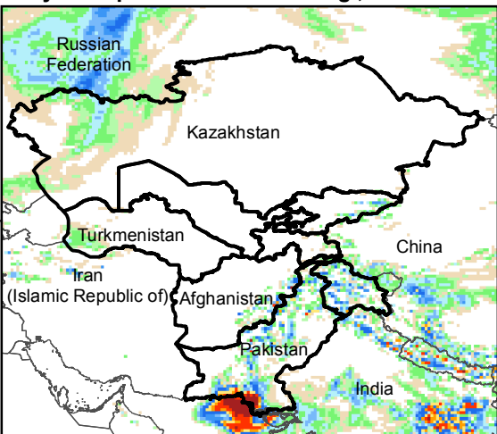
Daily Precip. Forecast for 14 Aug., 2019
