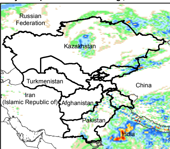
Daily Precip. Forecast for 15 Aug., 2019
