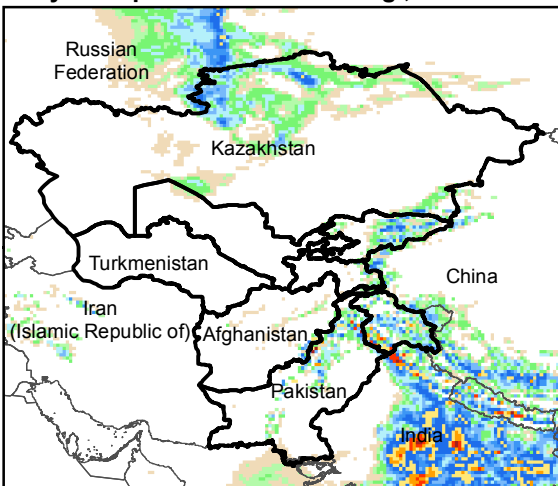
Daily Precip. Forecast for 16 Aug., 2019
