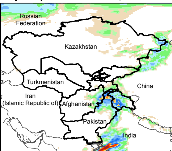
Daily Precip. Forecast for 6 Nov., 2019
