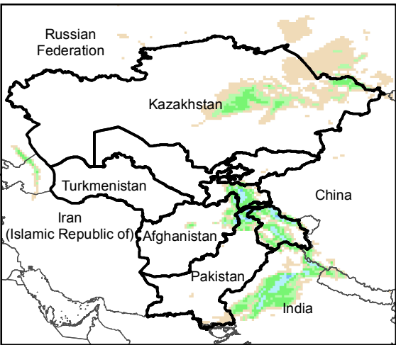
Daily Precip. Forecast for 26 Nov., 2019
