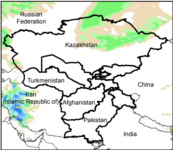
Daily Precip. Forecast for 3 Dec., 2019
