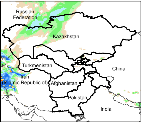
Daily Precip. Forecast for 2 Dec., 2019
