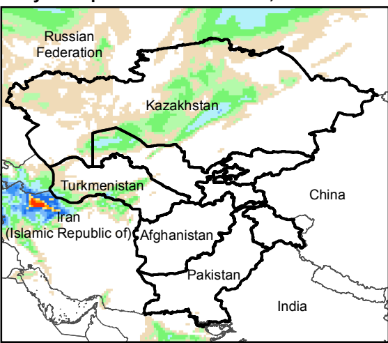
Daily Precip. Forecast for 5 Dec., 2019
