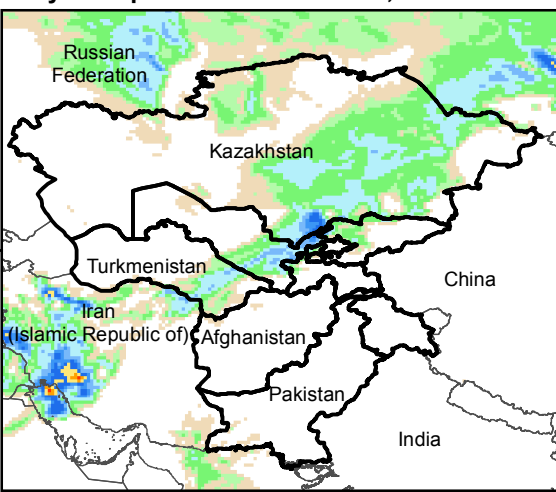
Daily Precip. Forecast for 6 Dec., 2019
