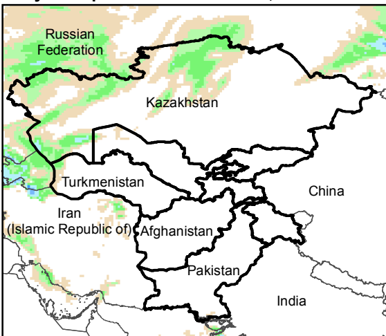
Daily Precip. Forecast for 7 Dec., 2019
