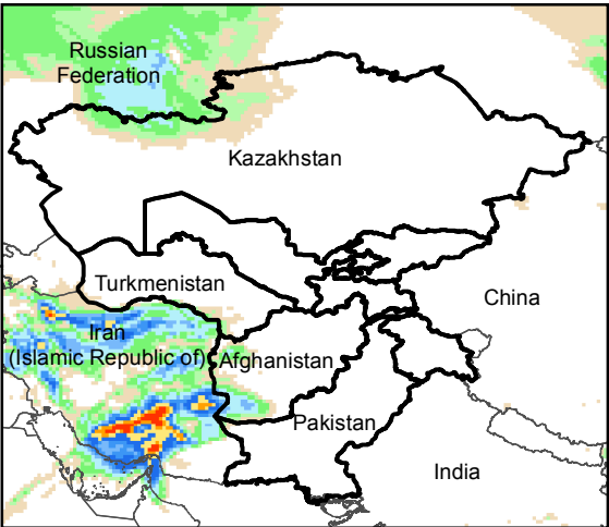
Daily Precip. Forecast for 17 Dec., 2019
