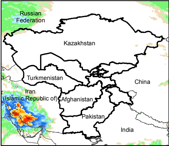
Daily Precip. Forecast for 19 Dec., 2019
