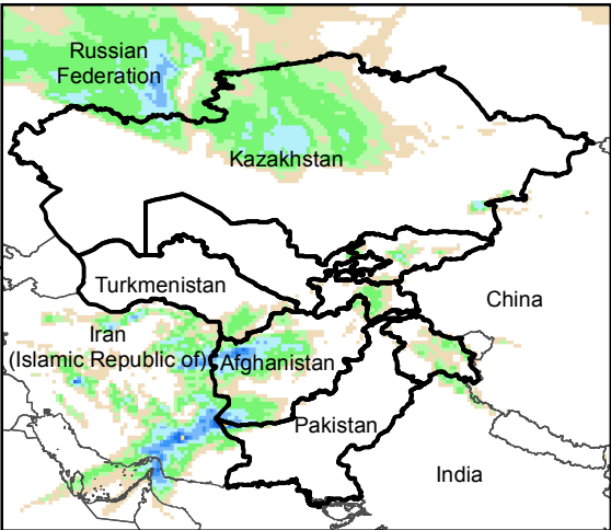
Daily Precip. Forecast for 18 Dec., 2019
