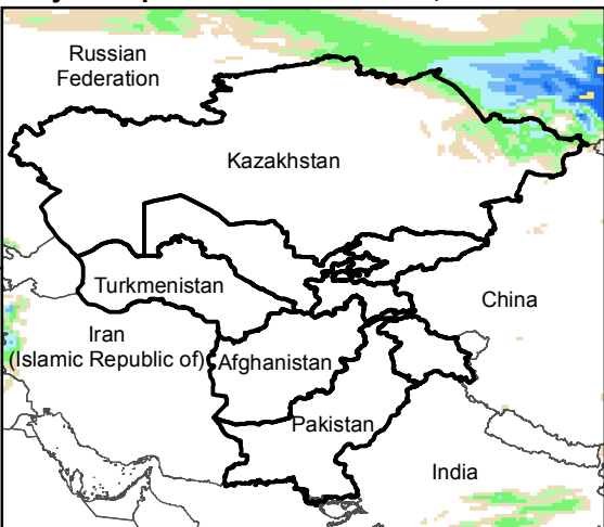
Daily Precip. Forecast for 28 Dec., 2019
