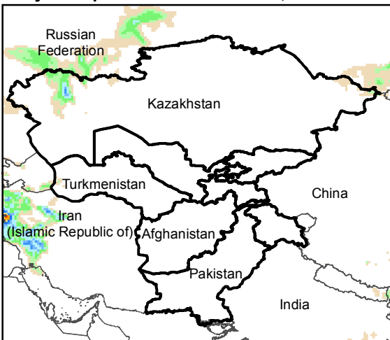
Daily Precip. Forecast for 30 Dec., 2019
