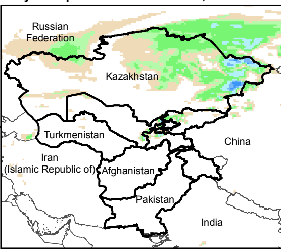
Daily Precip. Forecast for 29 Dec., 2019
