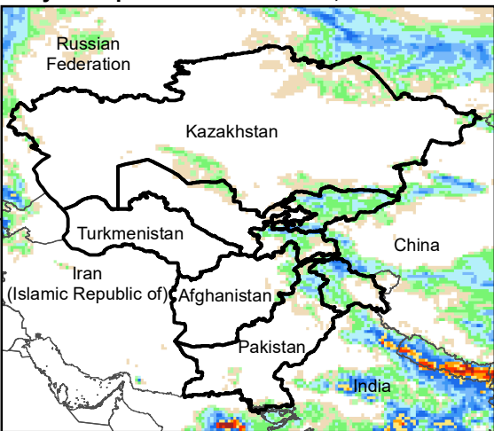
Daily Precip. Forecast for 12 Jul., 2020
