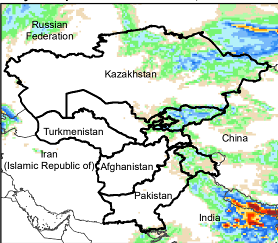
Daily Precip. Forecast for 13 Jul., 2020
