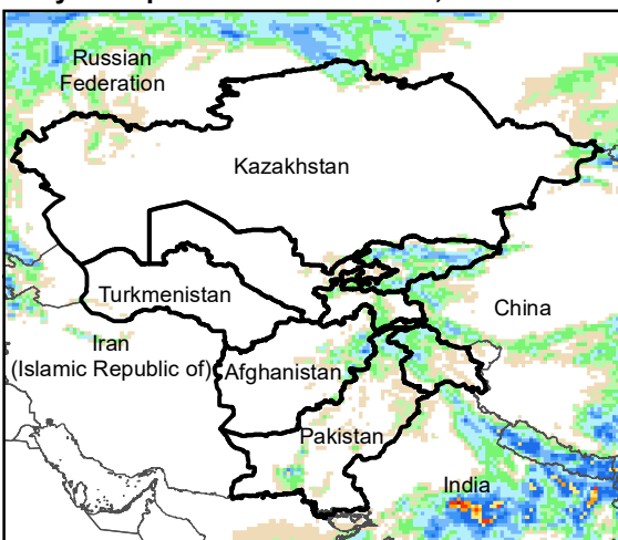
Daily Precip. Forecast for 14 Jul., 2020
