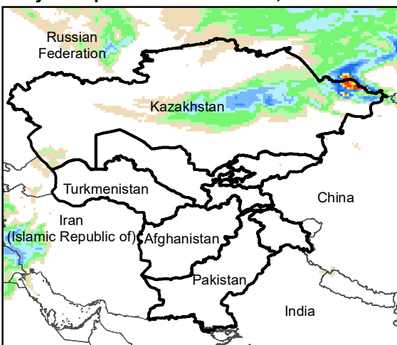
Daily Precip. Forecast for 9 Nov., 2020
