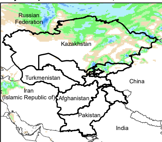
Daily Precip. Forecast for 8 Nov., 2020
