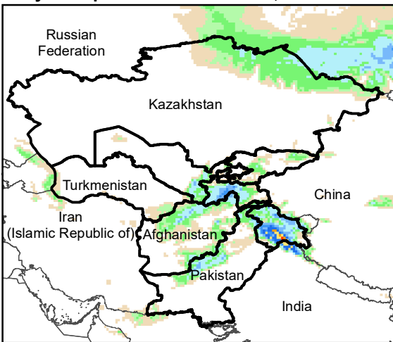
Daily Precip. Forecast for 11 Dec., 2020
