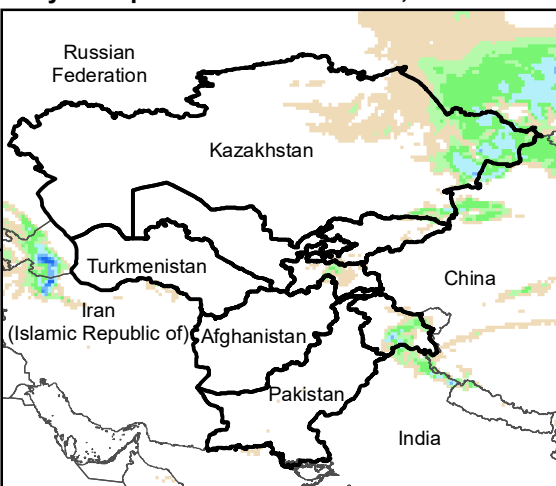
Daily Precip. Forecast for 10 Dec., 2020
