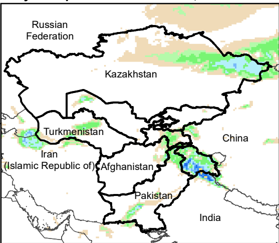
Daily Precip. Forecast for 12 Dec., 2020
