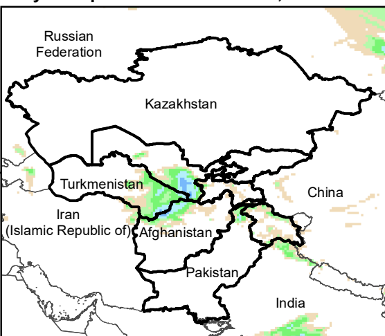
Daily Precip. Forecast for 13 Dec., 2020
