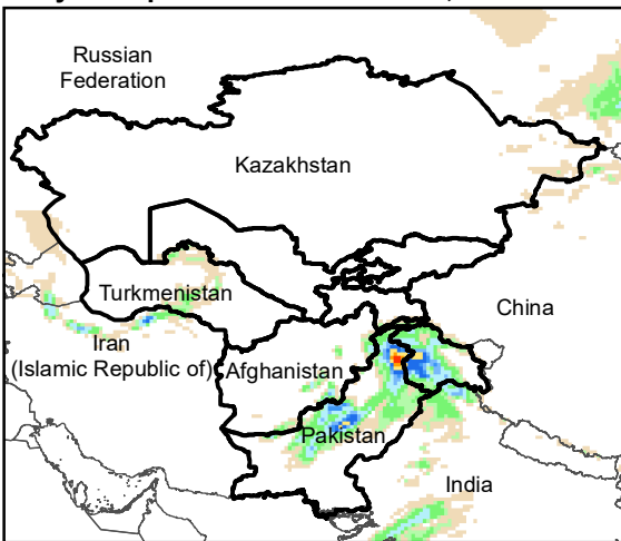
Daily Precip. Forecast for 14 Dec., 2020
