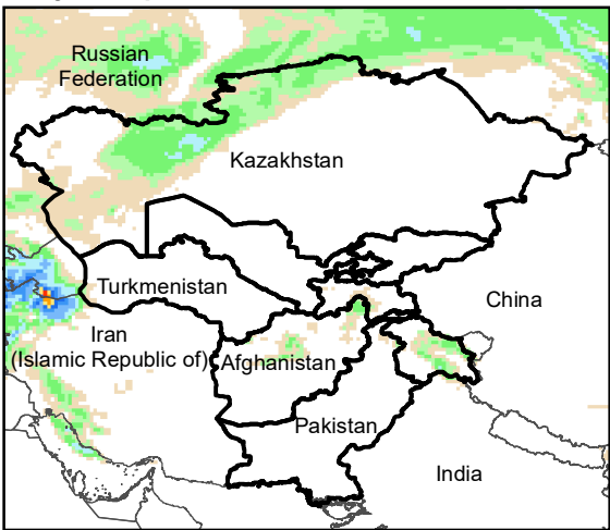
Daily Precip. Forecast for 18 Dec., 2020
