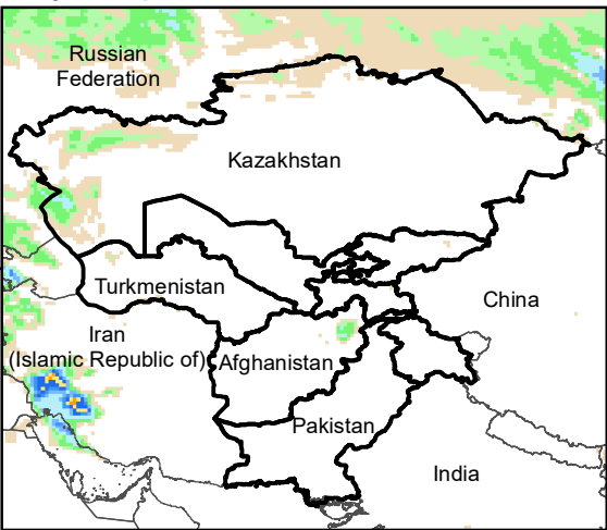
Daily Precip. Forecast for 17 Dec., 2020
