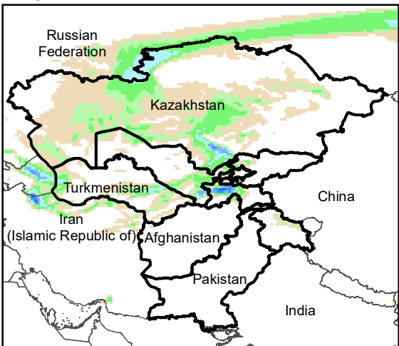
Daily Precip. Forecast for 19 Dec., 2020
