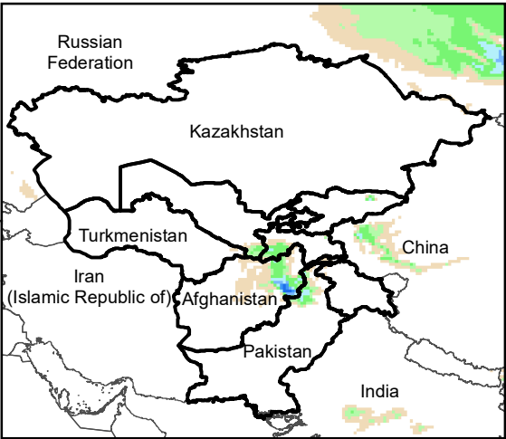
Daily Precip. Forecast for 17 Dec., 2020
