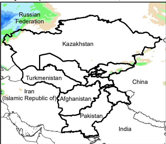
Daily Precip. Forecast for 17 Jan., 2021
