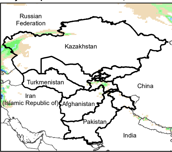
Daily Precip. Forecast for 18 Jan., 2021
