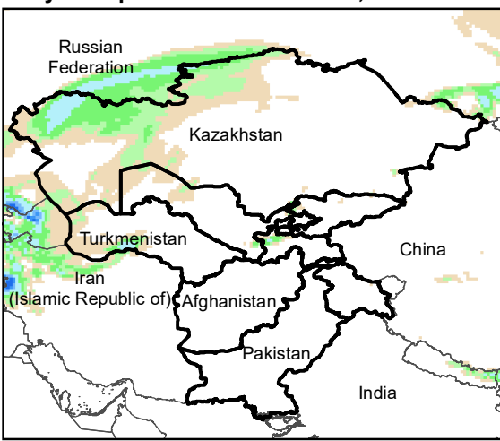
Daily Precip. Forecast for 19 Jan., 2021
