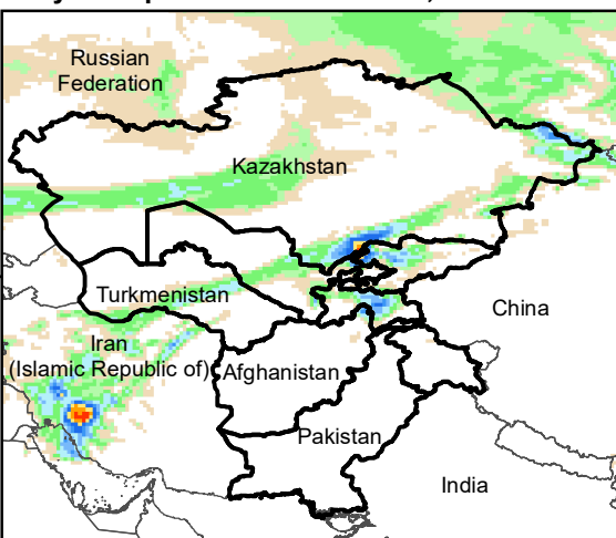
Daily Precip. Forecast for 7 Feb., 2021
