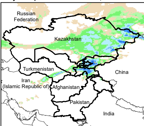
Daily Precip. Forecast for 8 Feb., 2021
