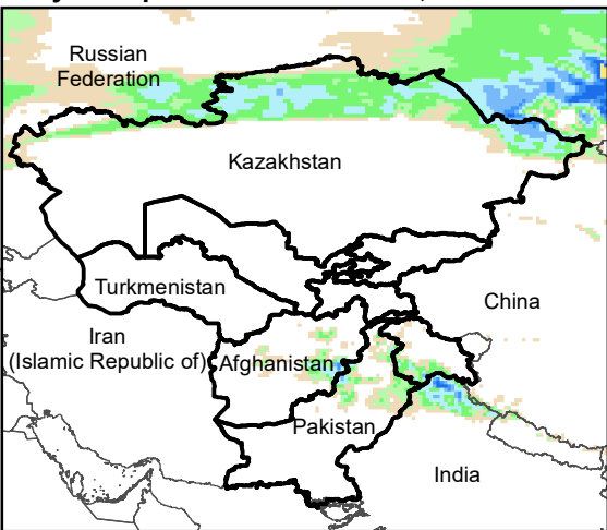
Daily Precip. Forecast for 6 Feb., 2021
