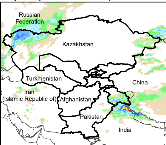
Daily Precip. Forecast for 26 Apr., 2021
