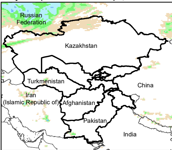
Daily Precip. Forecast for 28 Apr., 2021
