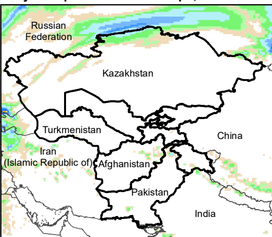
Daily Precip. Forecast for 27 Apr., 2021
