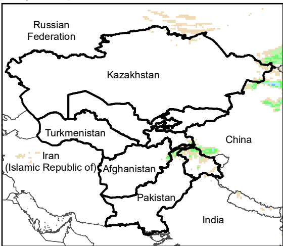
Daily Precip. Forecast for 13 Oct., 2021
