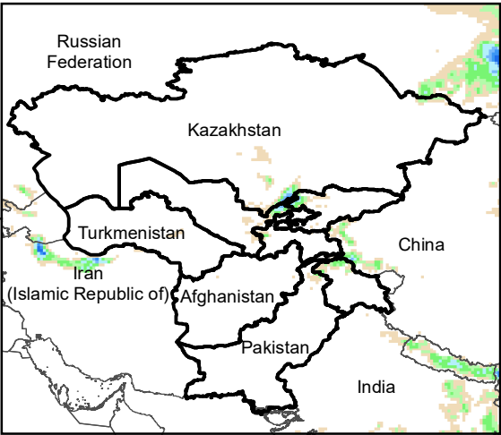
Daily Precip. Forecast for 11 Oct., 2021
