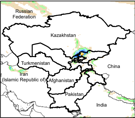
Daily Precip. Forecast for 12 Oct., 2021
