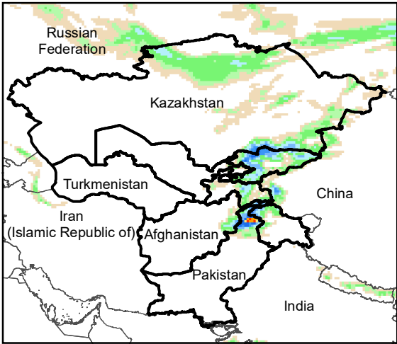
Daily Precip. Forecast for 13 Oct., 2021
