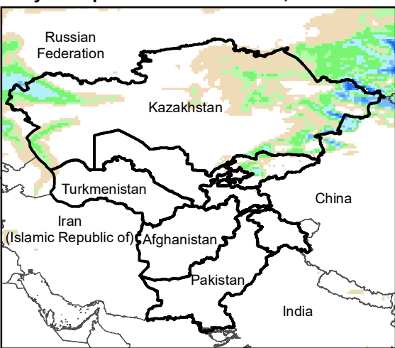
Daily Precip. Forecast for 15 Nov., 2021
