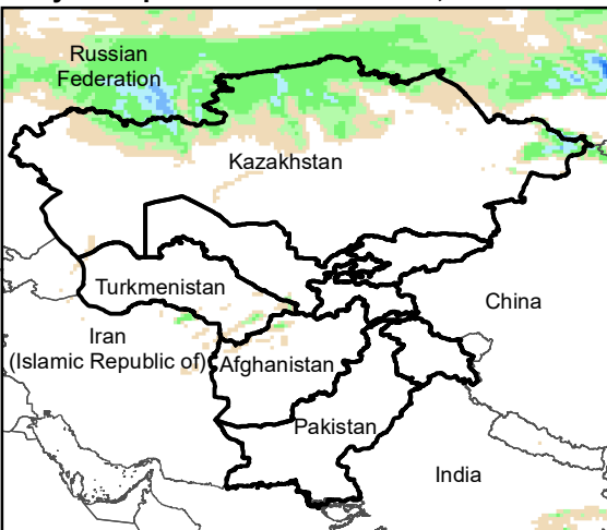
Daily Precip. Forecast for 16 Nov., 2021
