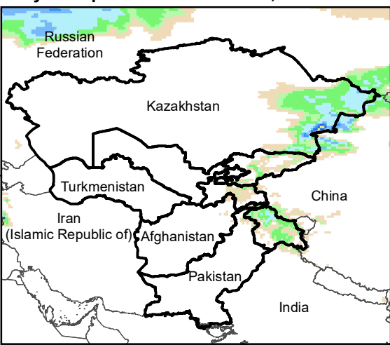
Daily Precip. Forecast for 8 Dec., 2021
