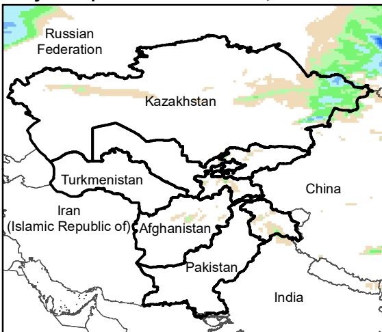
Daily Precip. Forecast for 10 Dec., 2021
