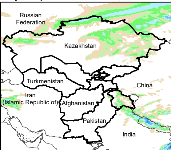
Daily Precip. Forecast for 9 Dec., 2021
