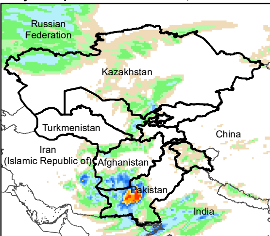
Daily Precip. Forecast for 9 Jan., 2022
