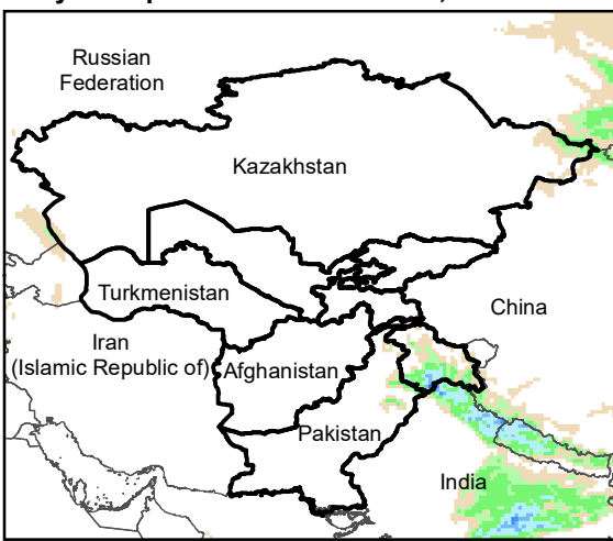
Daily Precip. Forecast for 10 Jan., 2022
