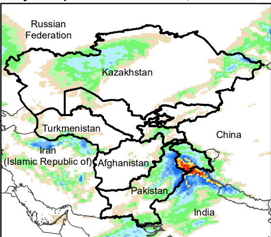
Daily Precip. Forecast for 8 Jan., 2022
