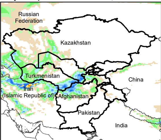
Daily Precip. Forecast for 8 Feb., 2022
