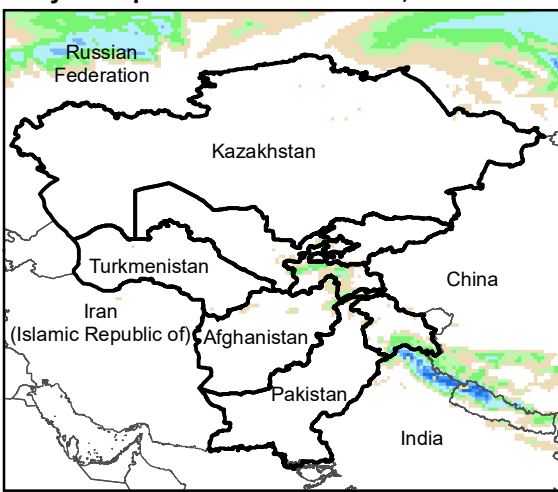
Daily Precip. Forecast for 23 Feb., 2022
