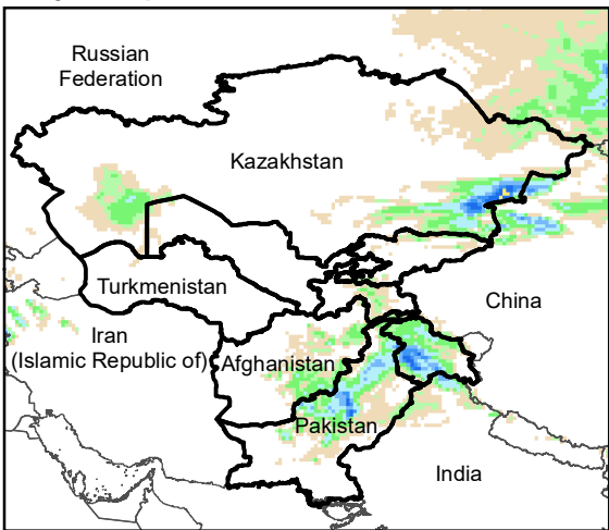
Daily Precip. Forecast for 2 Mar., 2022
