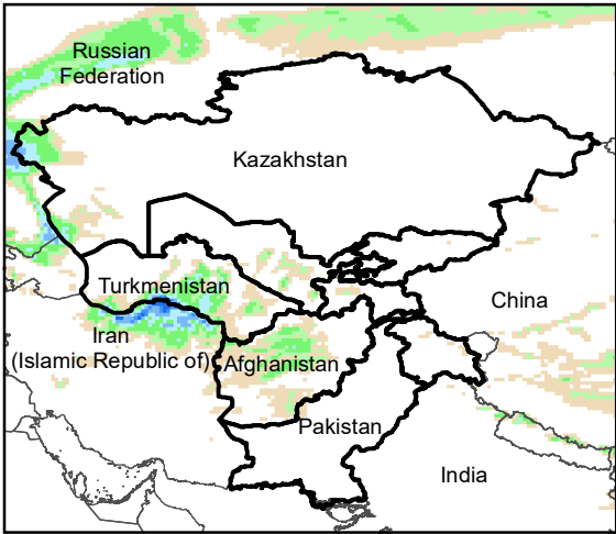
Daily Precip. Forecast for 2 Mar., 2022
