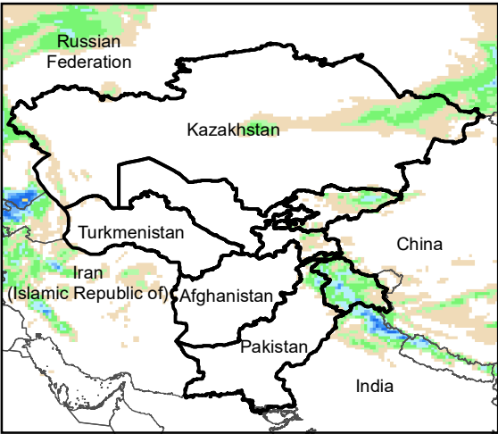
Daily Precip. Forecast for 1 Mar., 2022
