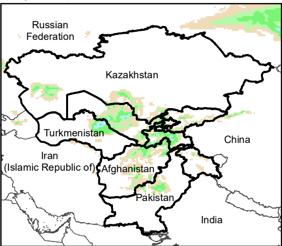
Daily Precip. Forecast for 28 Feb., 2022
