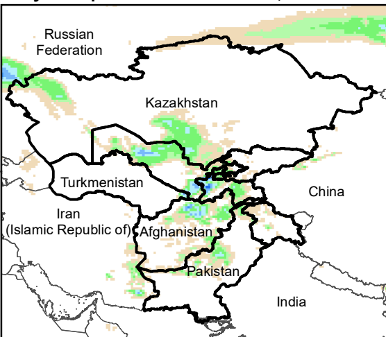
Daily Precip. Forecast for 3 Mar., 2022
