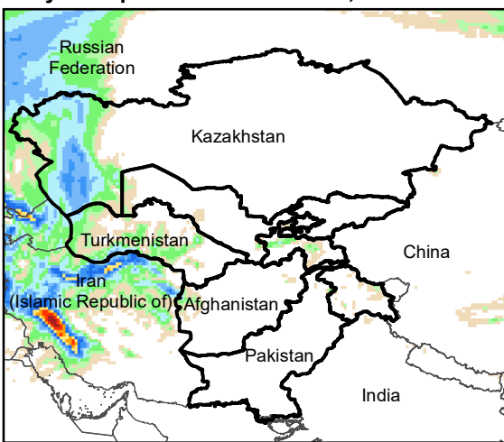
Daily Precip. Forecast for 4 Mar., 2022
