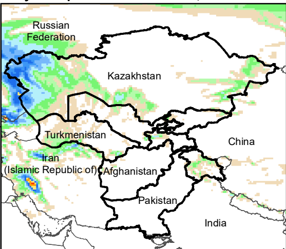
Daily Precip. Forecast for 7 Mar., 2022
