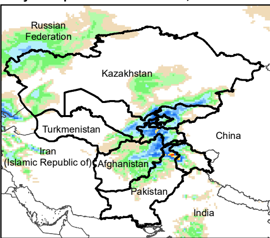
Daily Precip. Forecast for 9 Mar., 2022
