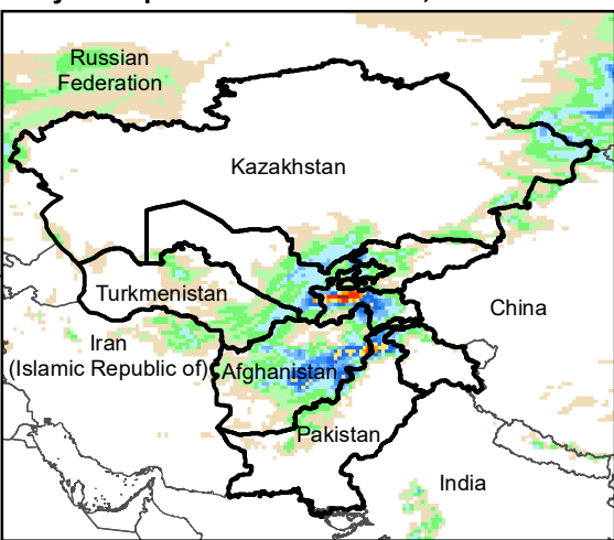
Daily Precip. Forecast for 8 Mar., 2022
