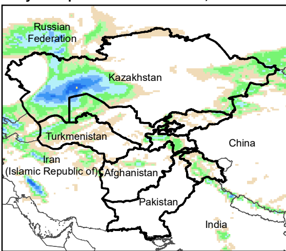
Daily Precip. Forecast for 10 Mar., 2022
