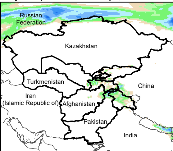
Daily Precip. Forecast for 5 Apr., 2022
