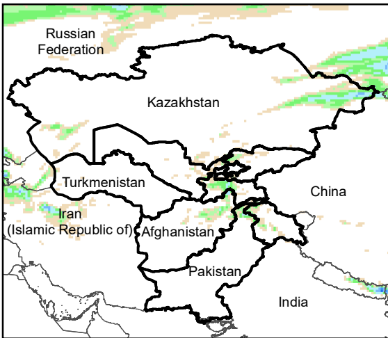
Daily Precip. Forecast for 7 Apr., 2022
