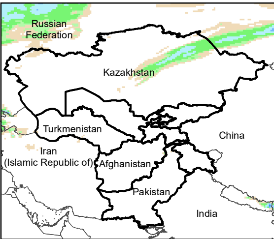
Daily Precip. Forecast for 6 Apr., 2022
