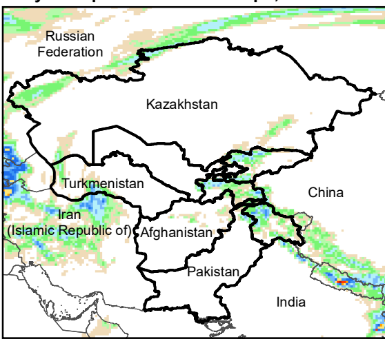
Daily Precip. Forecast for 30 Apr., 2022
