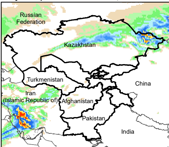
Daily Precip. Forecast for 8 Jan., 2023
