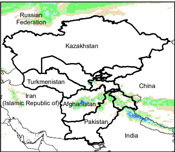
Daily Precip. Forecast for 25 Mar., 2023
