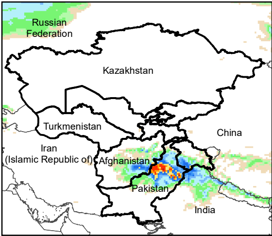
Daily Precip. Forecast for 27 Mar., 2023
