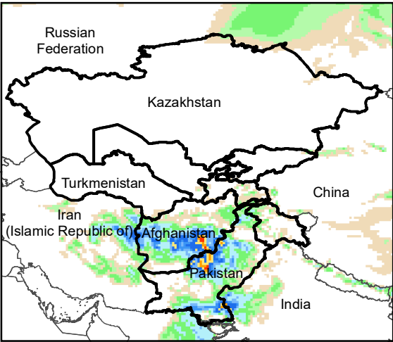
Daily Precip. Forecast for 26 Mar., 2023
