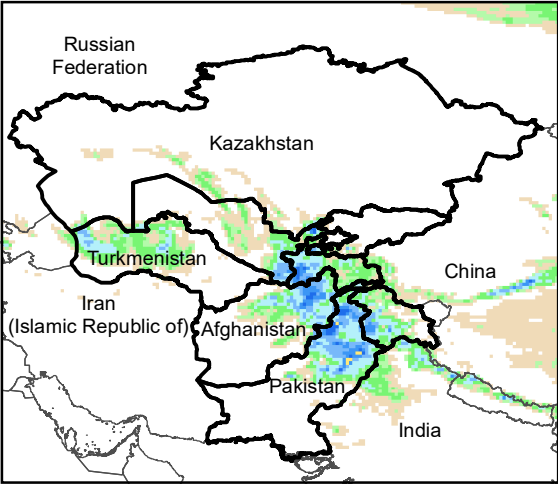
Daily Precip. Forecast for 6 Apr., 2023
