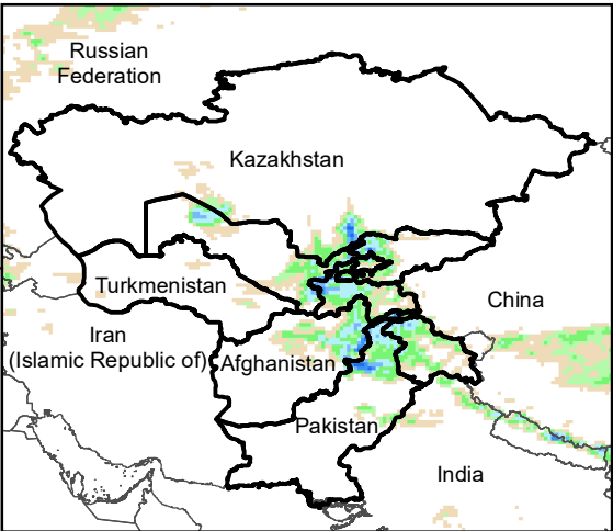
Daily Precip. Forecast for 5 Apr., 2023
