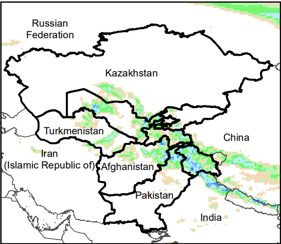
Daily Precip. Forecast for 7 Apr., 2023
