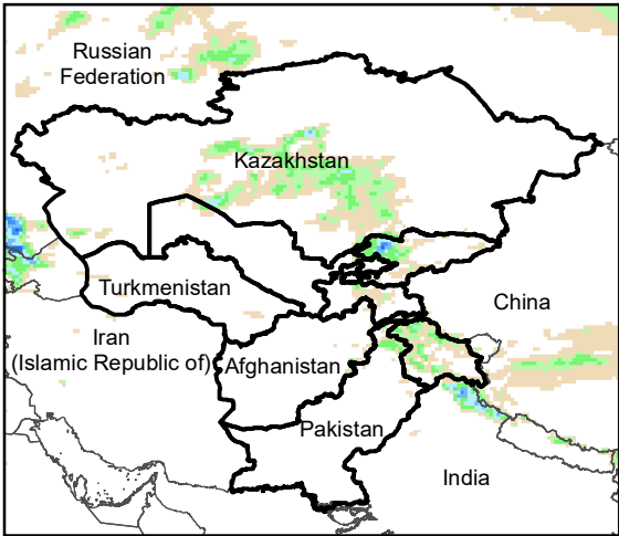
Daily Precip. Forecast for 9 Apr., 2023
