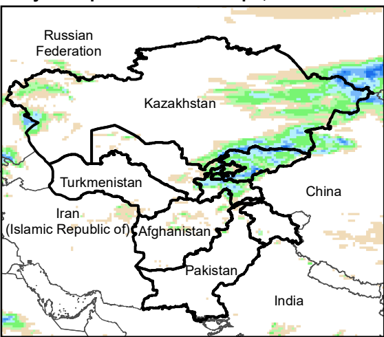
Daily Precip. Forecast for 8 Apr., 2023
