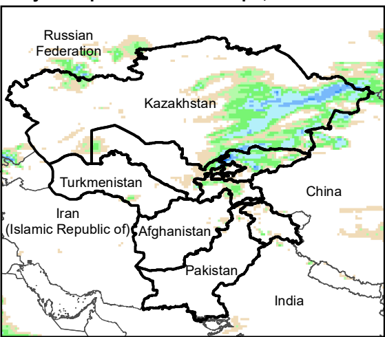
Daily Precip. Forecast for 7 Apr., 2023
