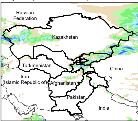
Daily Precip. Forecast for 9 Apr., 2023
