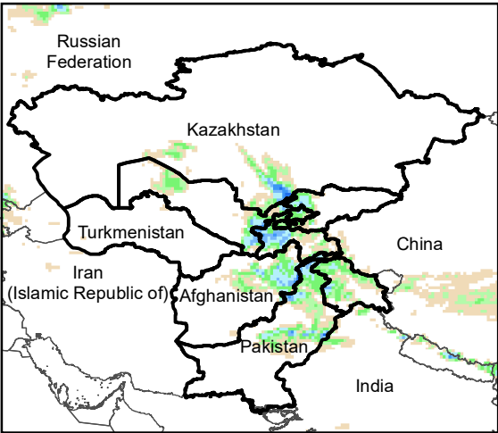
Daily Precip. Forecast for 8 Apr., 2023
