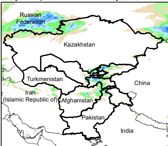
Daily Precip. Forecast for 15 May., 2023
