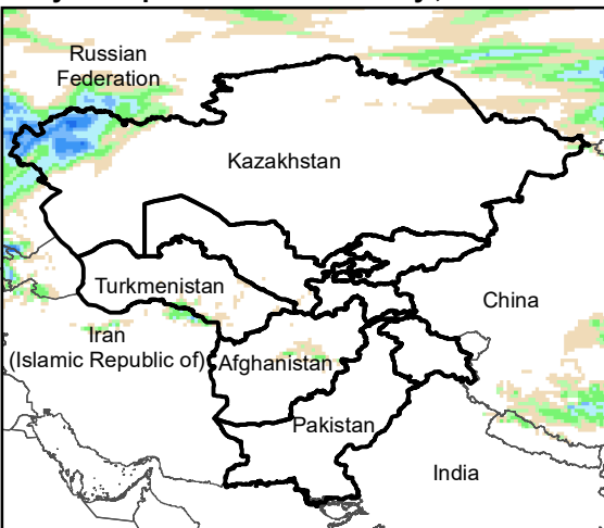
Daily Precip. Forecast for 14 May., 2023
