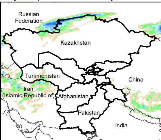
Daily Precip. Forecast for 13 May., 2023
