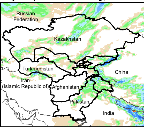
Daily Precip. Forecast for 26 Aug., 2023
