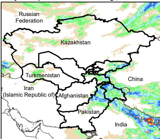
Daily Precip. Forecast for 28 Aug., 2023
