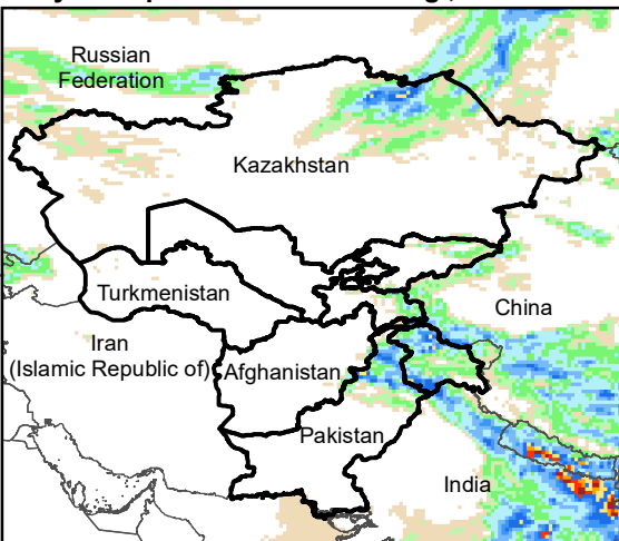
Daily Precip. Forecast for 27 Aug., 2023
