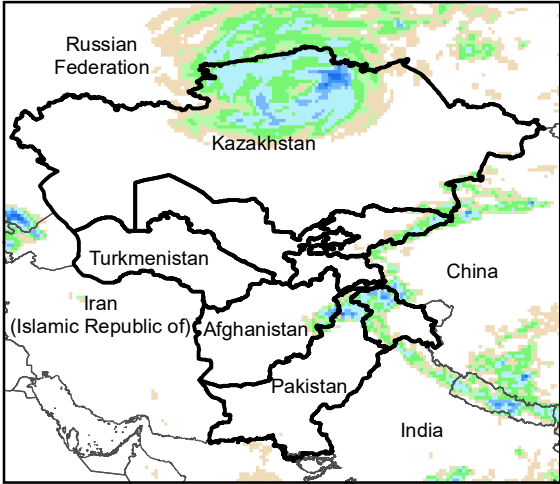
Daily Precip. Forecast for 5 Sep., 2023
