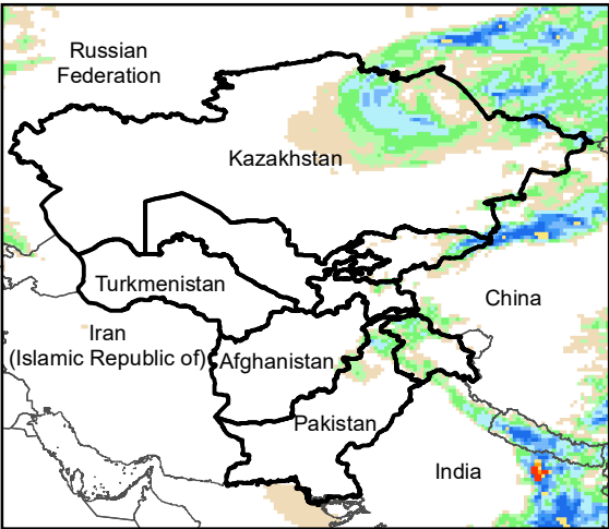
Daily Precip. Forecast for 4 Sep., 2023
