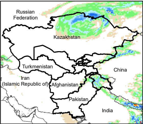
Daily Precip. Forecast for 3 Sep., 2023
