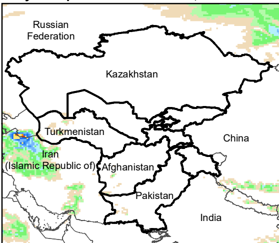
Daily Precip. Forecast for 7 Nov., 2023
