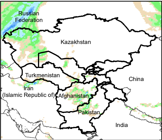
Daily Precip. Forecast for 7 Nov., 2023
