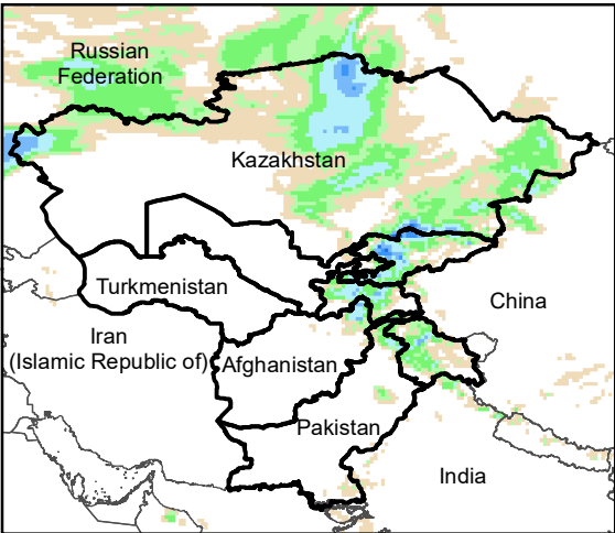
Daily Precip. Forecast for 9 Nov., 2023
