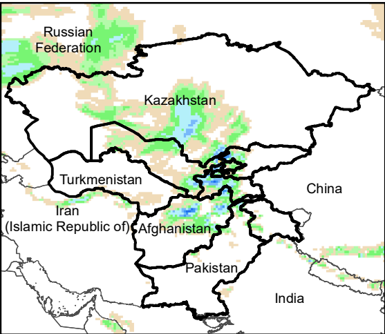
Daily Precip. Forecast for 8 Nov., 2023
