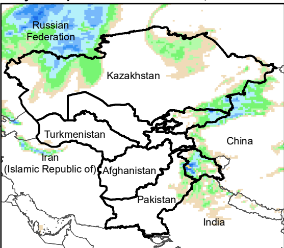
Daily Precip. Forecast for 13 Nov., 2023
