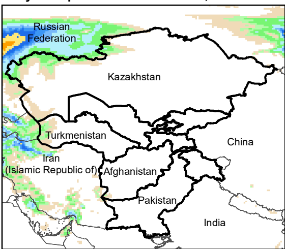
Daily Precip. Forecast for 17 Nov., 2023
