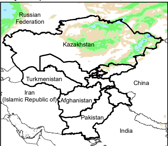
Daily Precip. Forecast for 15 Nov., 2023
