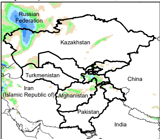
Daily Precip. Forecast for 27 Dec., 2023
