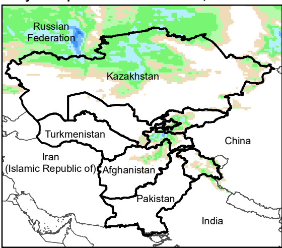
Daily Precip. Forecast for 27 Dec., 2023
