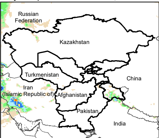
Daily Precip. Forecast for 26 Dec., 2023
