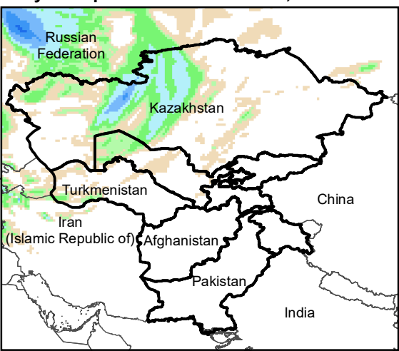
Daily Precip. Forecast for 25 Dec., 2023
